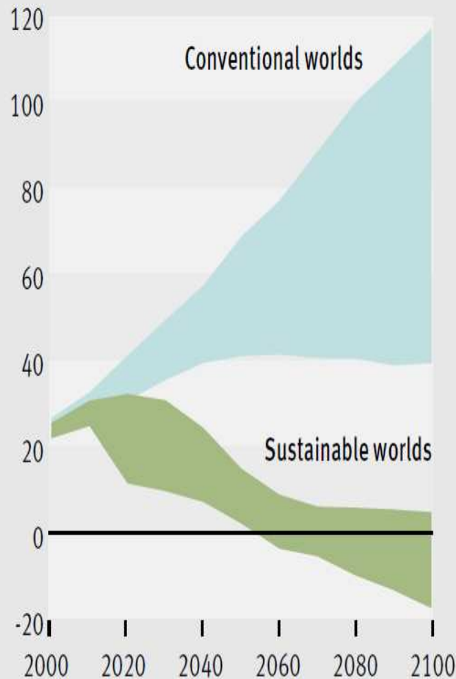
CO 2 emissions, billion tonnes
