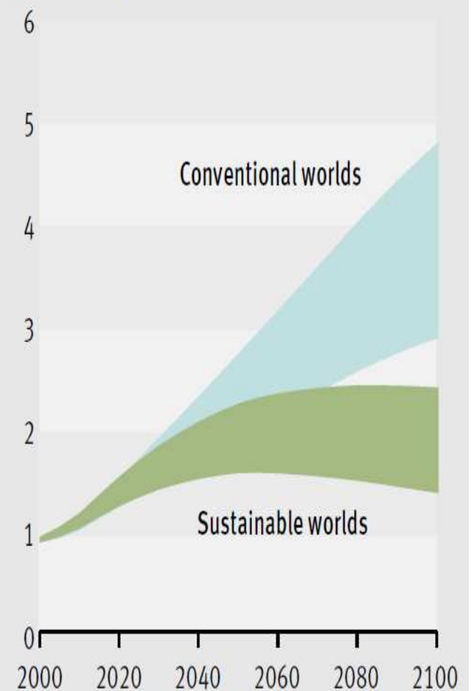
Temperature increase relative to pre-industrial levels, °C
