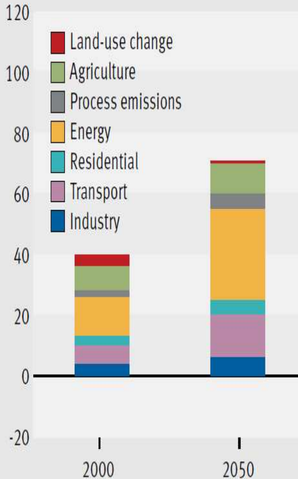
Annual emissions of CO 2 -equivalent by sector, billion tonnes
